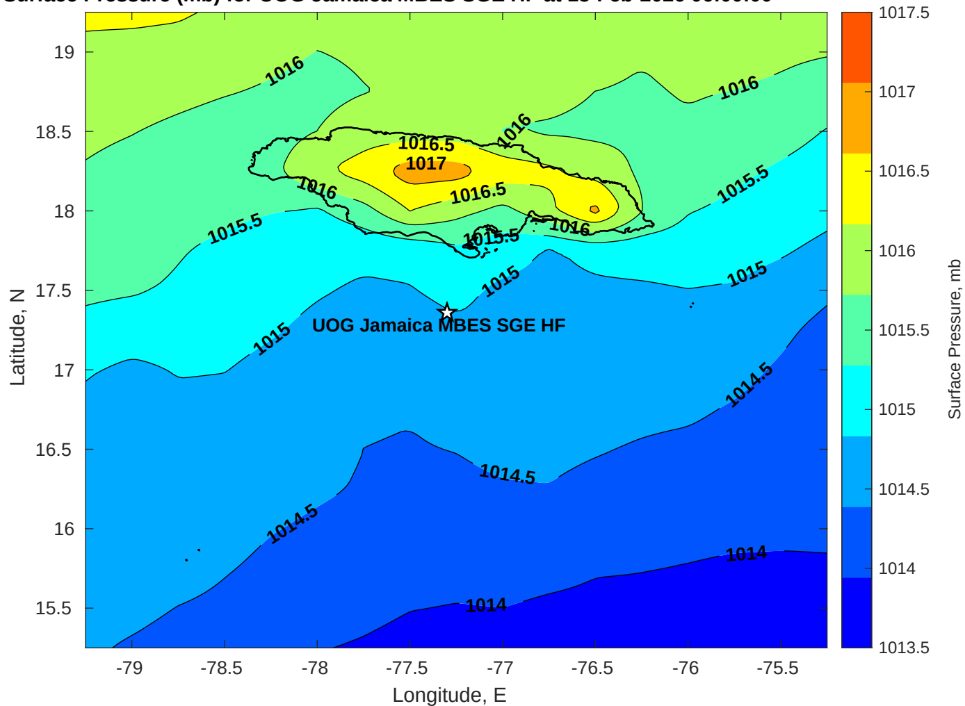
Surface Pressure (mb) for UOG Jamaica MBES SGE HF at 13-Feb-2026 06:00:00
