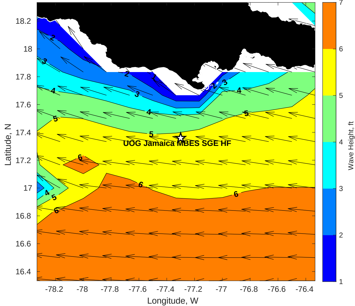
GFS Wave Height (ft) for UOG Jamaica MBES SGE HF at 12-Feb-2026 09:00:00
