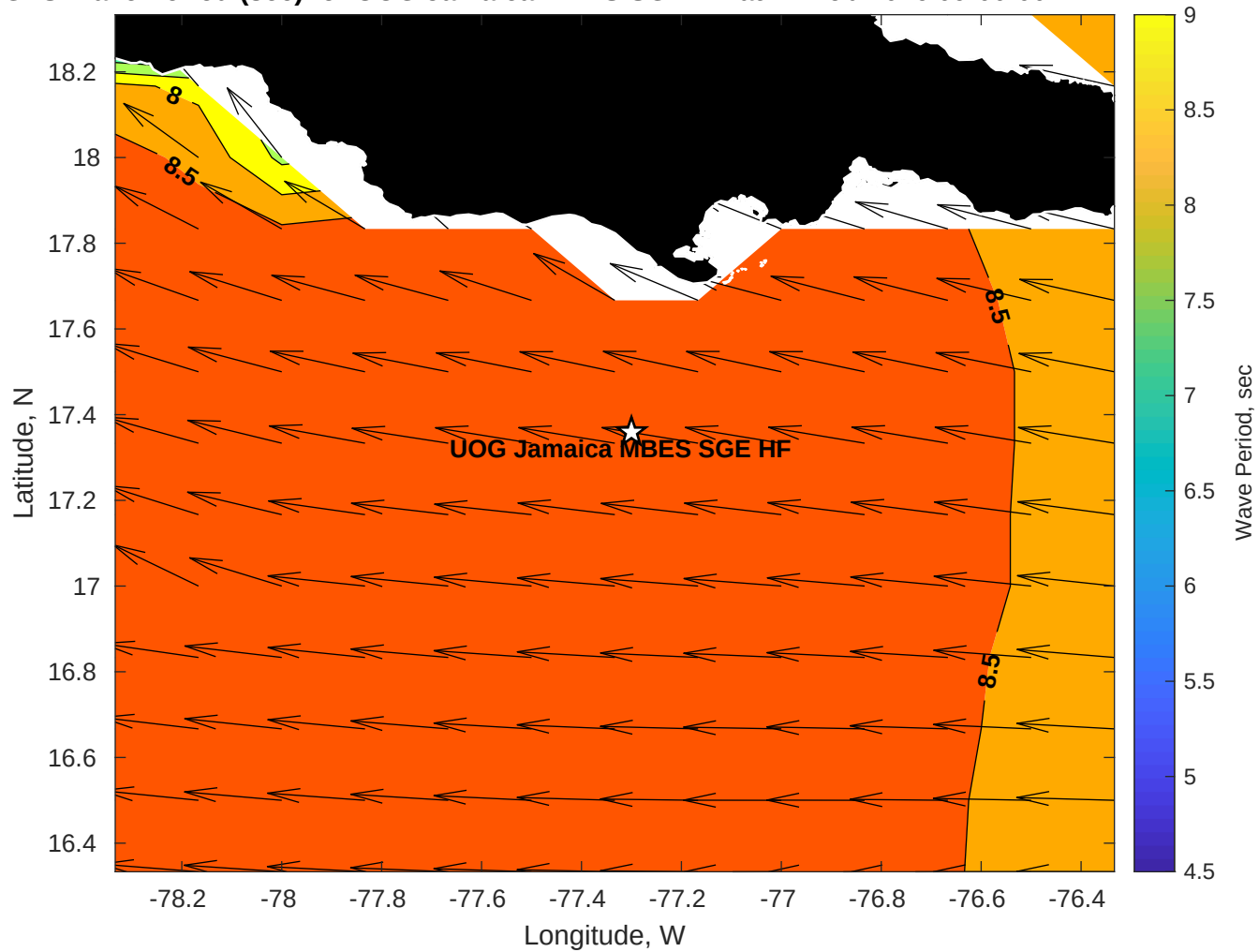
GFS Wave Period (sec) for UOG Jamaica MBES SGE HF at 12-Feb-2026 09:00:00
