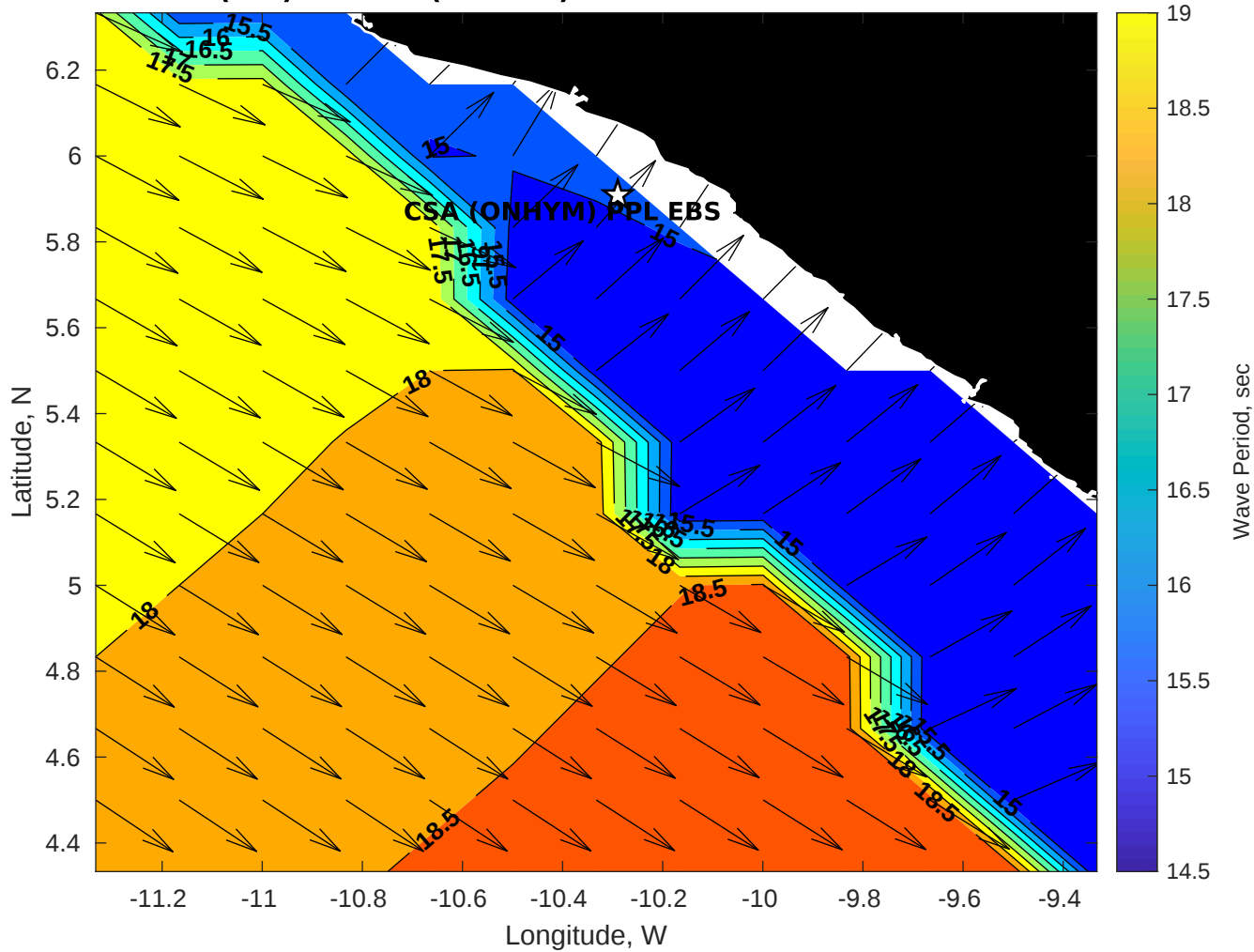
GFS Wave Period (sec) for CSA (ONHYM) PPL EBS - Liberia at 13-Feb-2026 09:00:00
