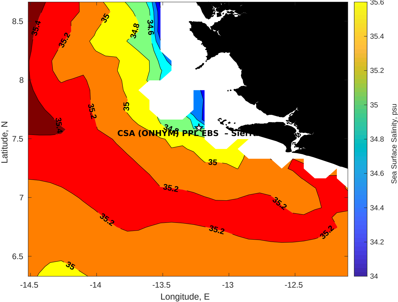
Surface Salinity for CSA (ONHYM) PPL EBS - Sierra Leone at 12-Feb-2026 00:00:00
