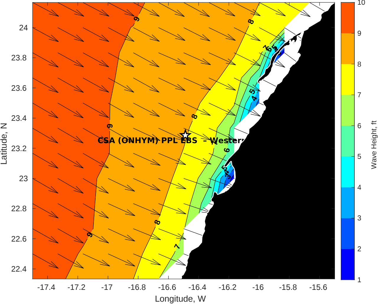
GFS Wave Height (ft) for CSA (ONHYM) PPL EBS - Western Sahara at 13-Feb-2026 09:00:00
