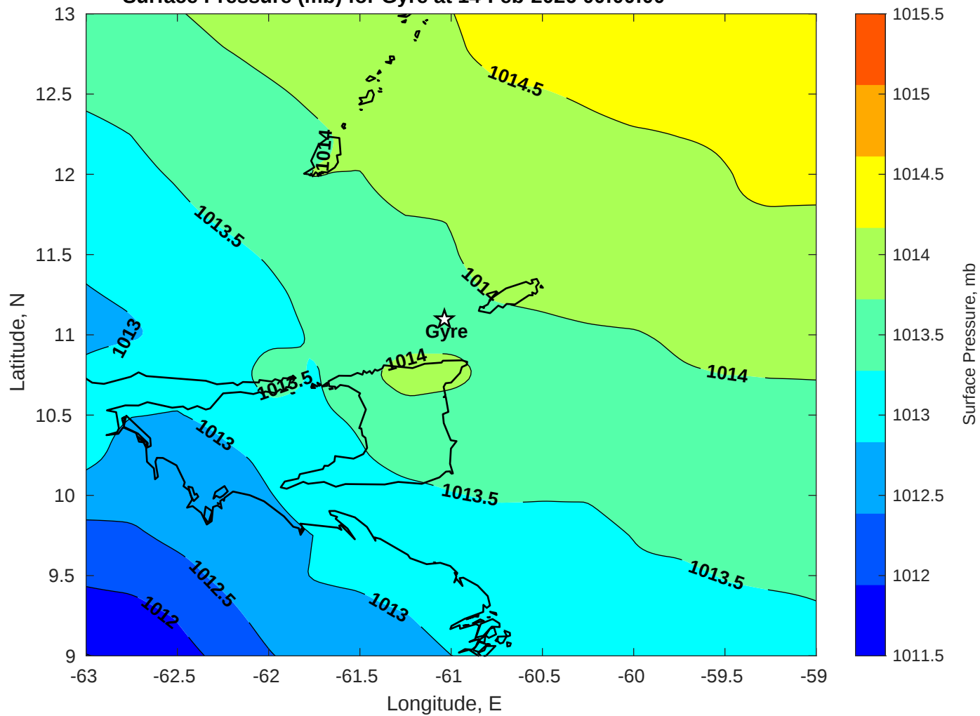
Surface Pressure (mb) for Gyre at 14-Feb-2026 00:00:00
