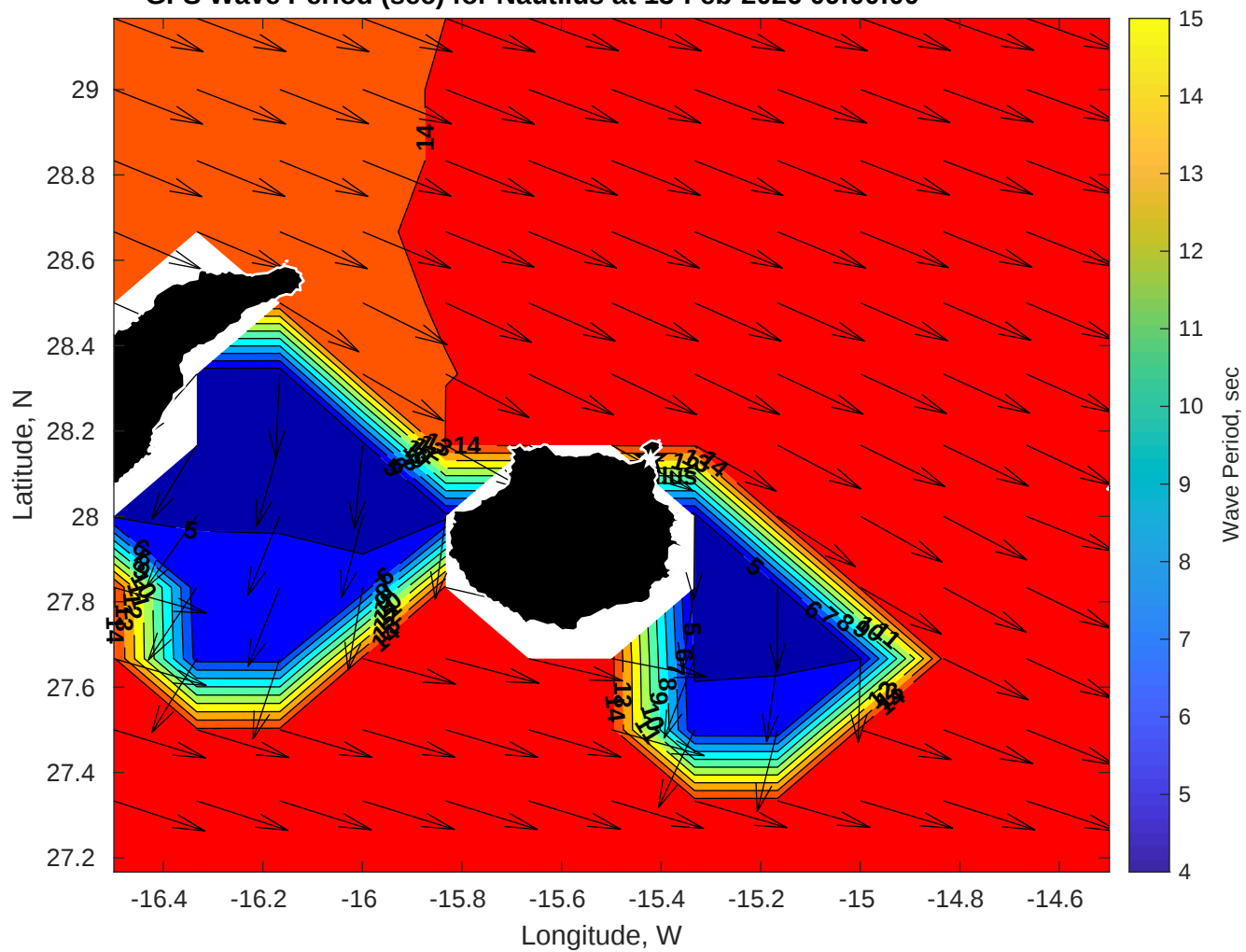
GFS Wave Period (sec) for Nautilus at 13-Feb-2026 09:00:00
