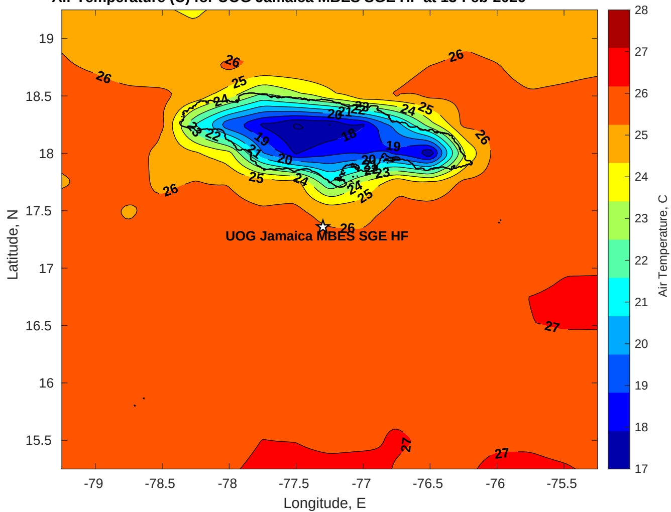
Air Temperature (C) for UOG Jamaica MBES SGE HF at 13-Feb-2026
