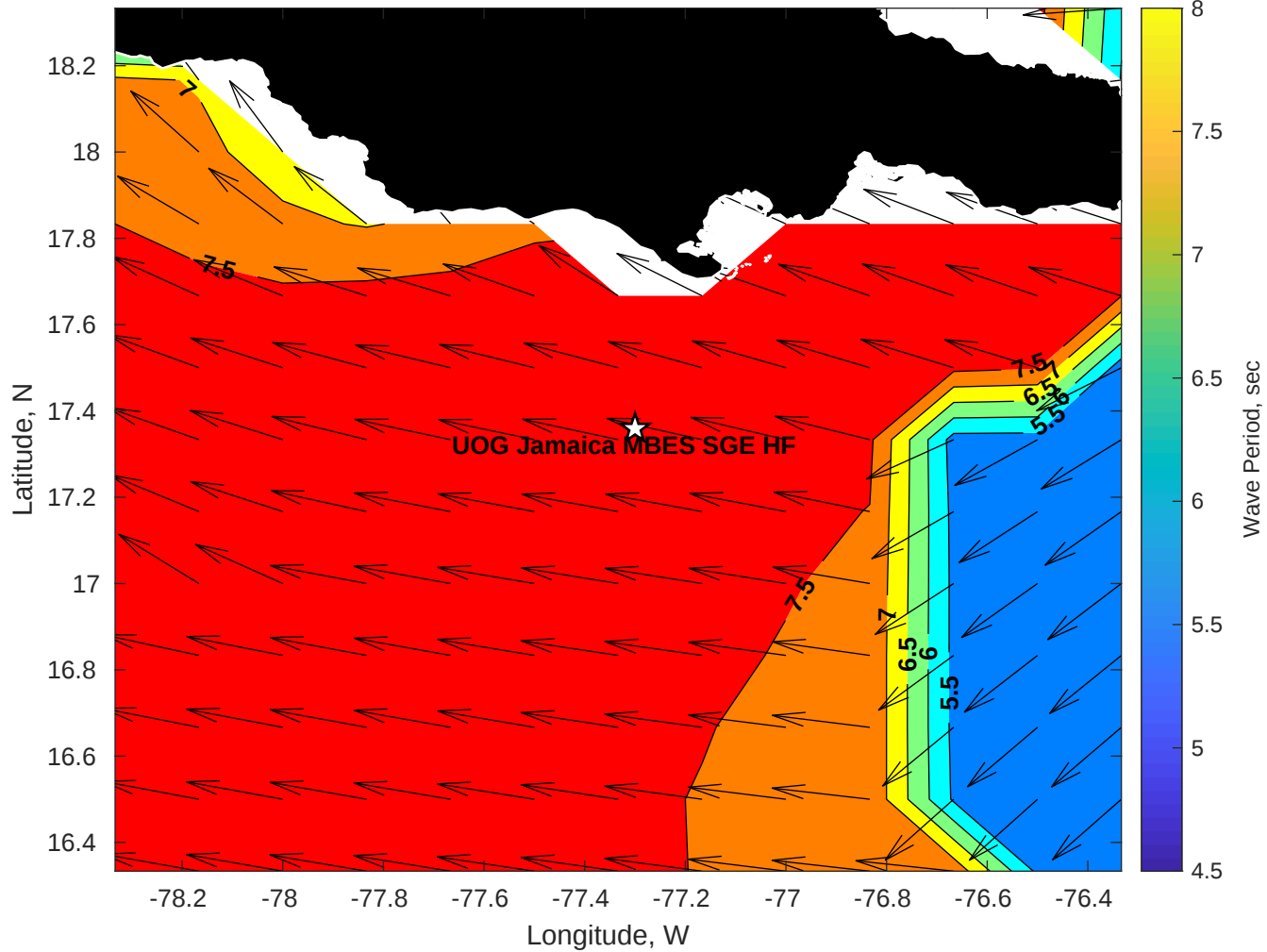
GFS Wave Period (sec) for UOG Jamaica MBES SGE HF at 13-Feb-2026 09:00:00
