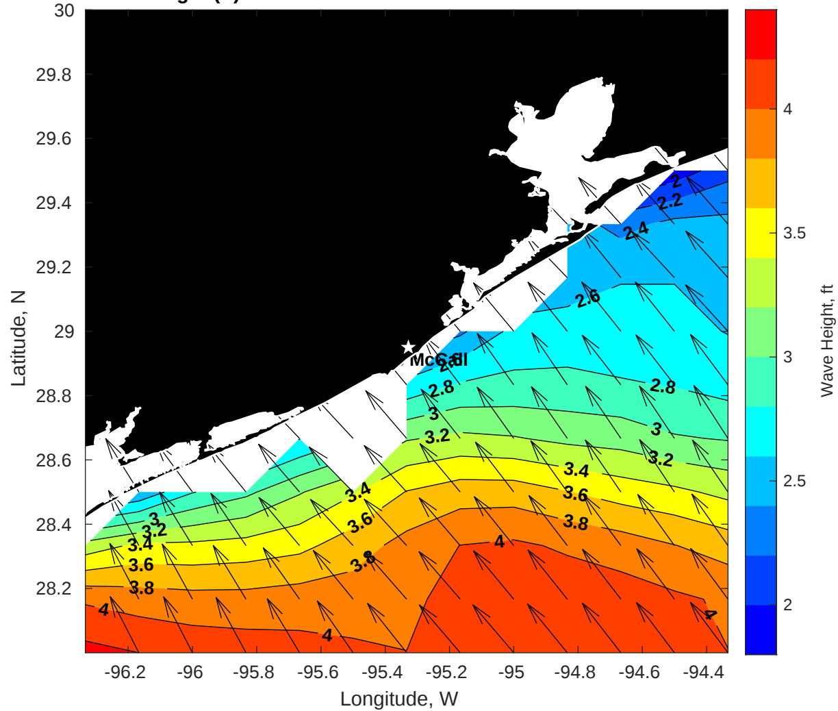
GFS Wave Height (ft) for Brooks McCall at 14-Feb-2026 09:00:00
