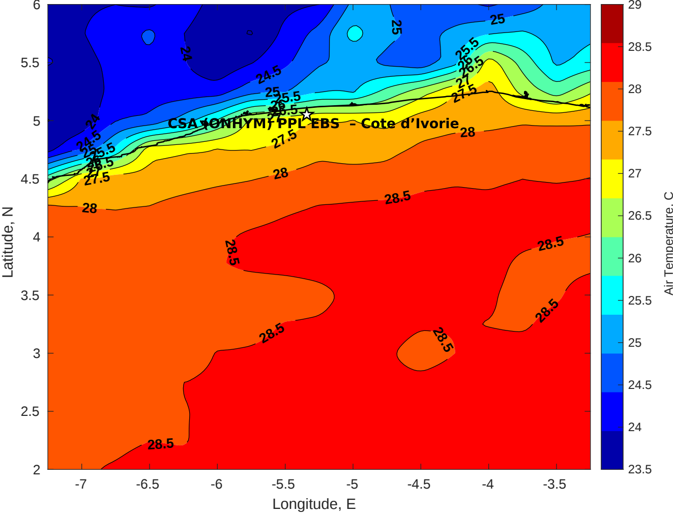
Air Temperature (C) for CSA (ONHYM) PPL EBS - Cote d'Ivoire at 14-Feb-2026
