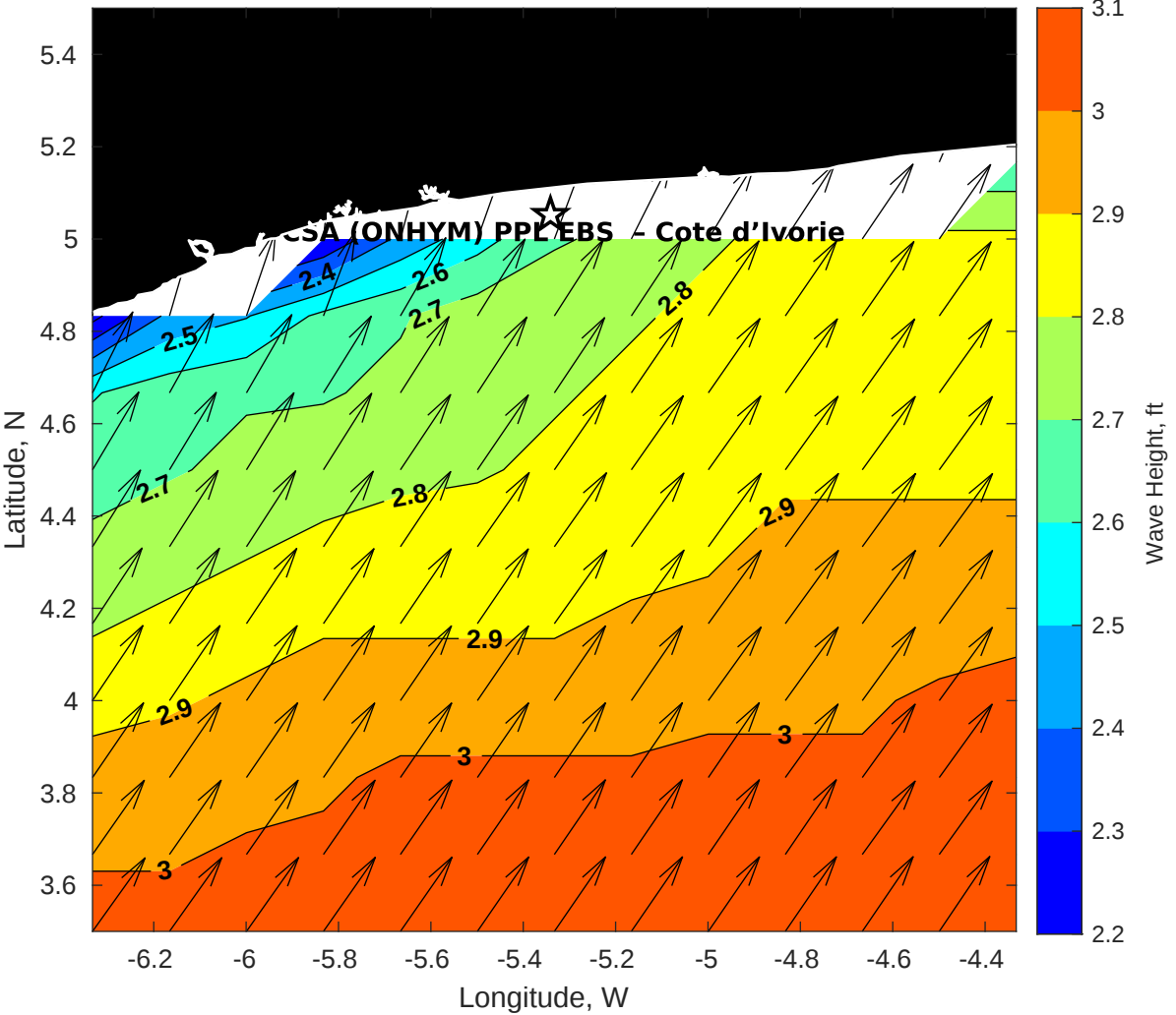
GFS Wave Height (ft) for CSA (ONHYM) PPL EBS - Cote d'Ivoire at 14-Feb-2026 09:00:00
