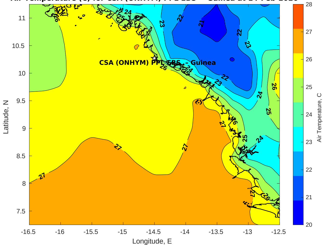
Air Temperature (C) for CSA (ONHYM) PPL EBS - Guinea at 14-Feb-2026
