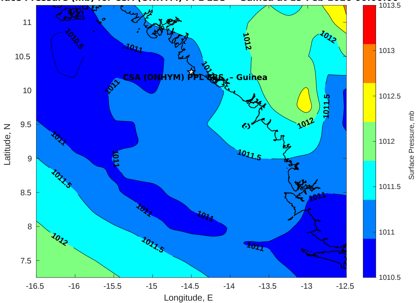
Surface Pressure (mb) for CSA (ONHYM) PPL EBS - Guinea at 15-Feb-2026 00:00:00
