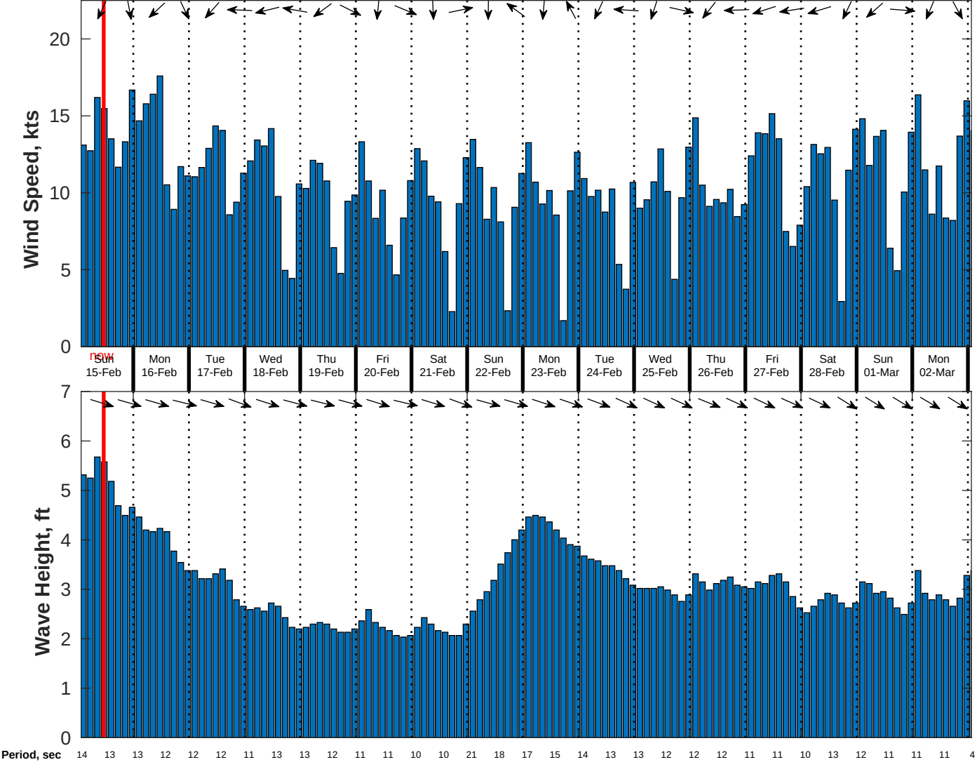
Wind & Wave Forecast for CSA (ONHYM) PPL EBS - Mauritania from 14-Feb-2026 01:00:00 to 02-Mar-2026 01:00:00
