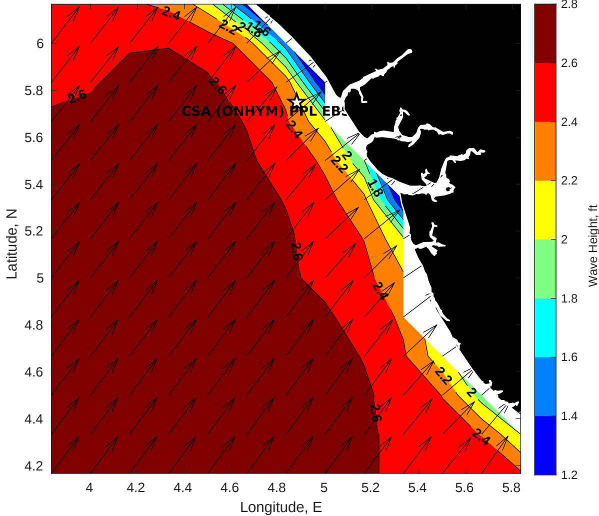
GFS Wave Height (ft) for CSA (ONHYM) PPL EBS - Nigeria at 14-Feb-2026 09:00:00
