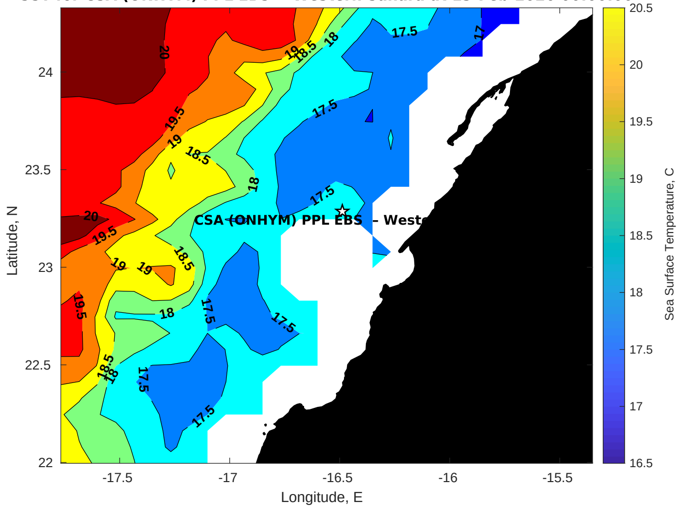
SST for CSA (ONHYM) PPL EBS - Western Sahara at 13-Feb-2026 00:00:00
