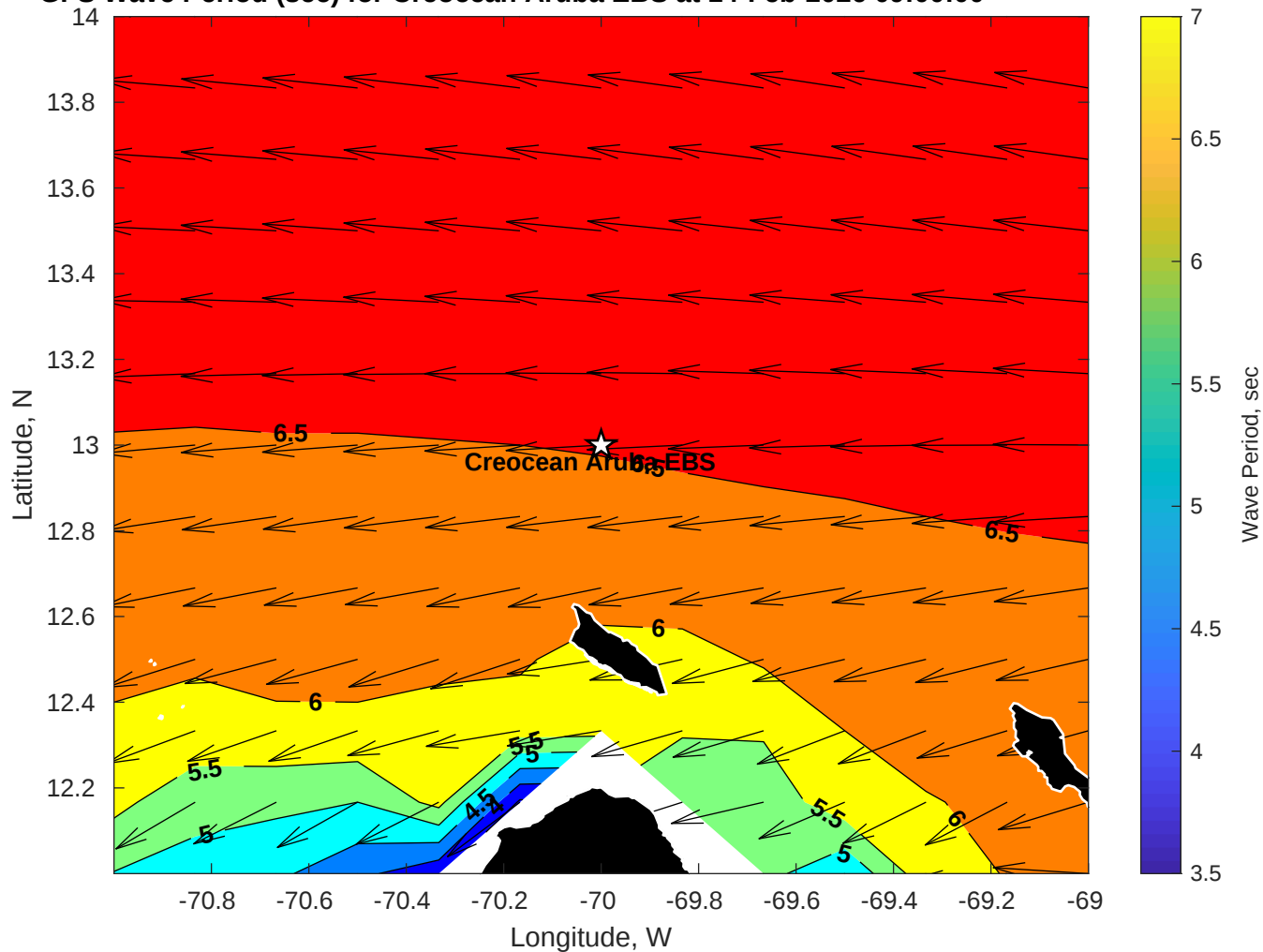
GFS Wave Period (sec) for Creoccean Aruba EBS at 14-Feb-2026 09:00:00
