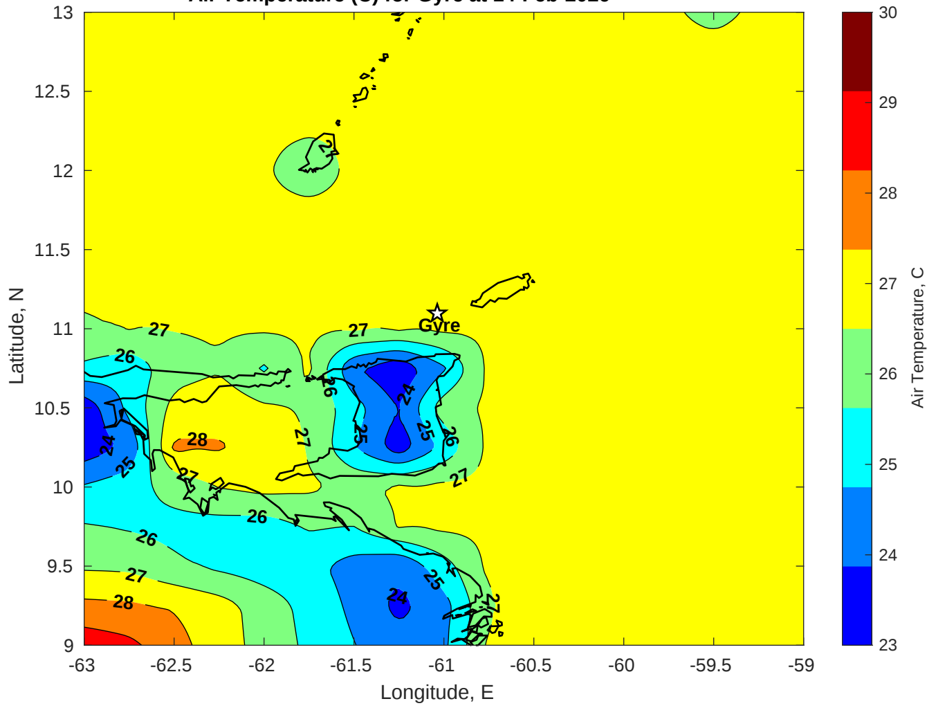
Air Temperature (C) for Gyre at 14-Feb-2026
