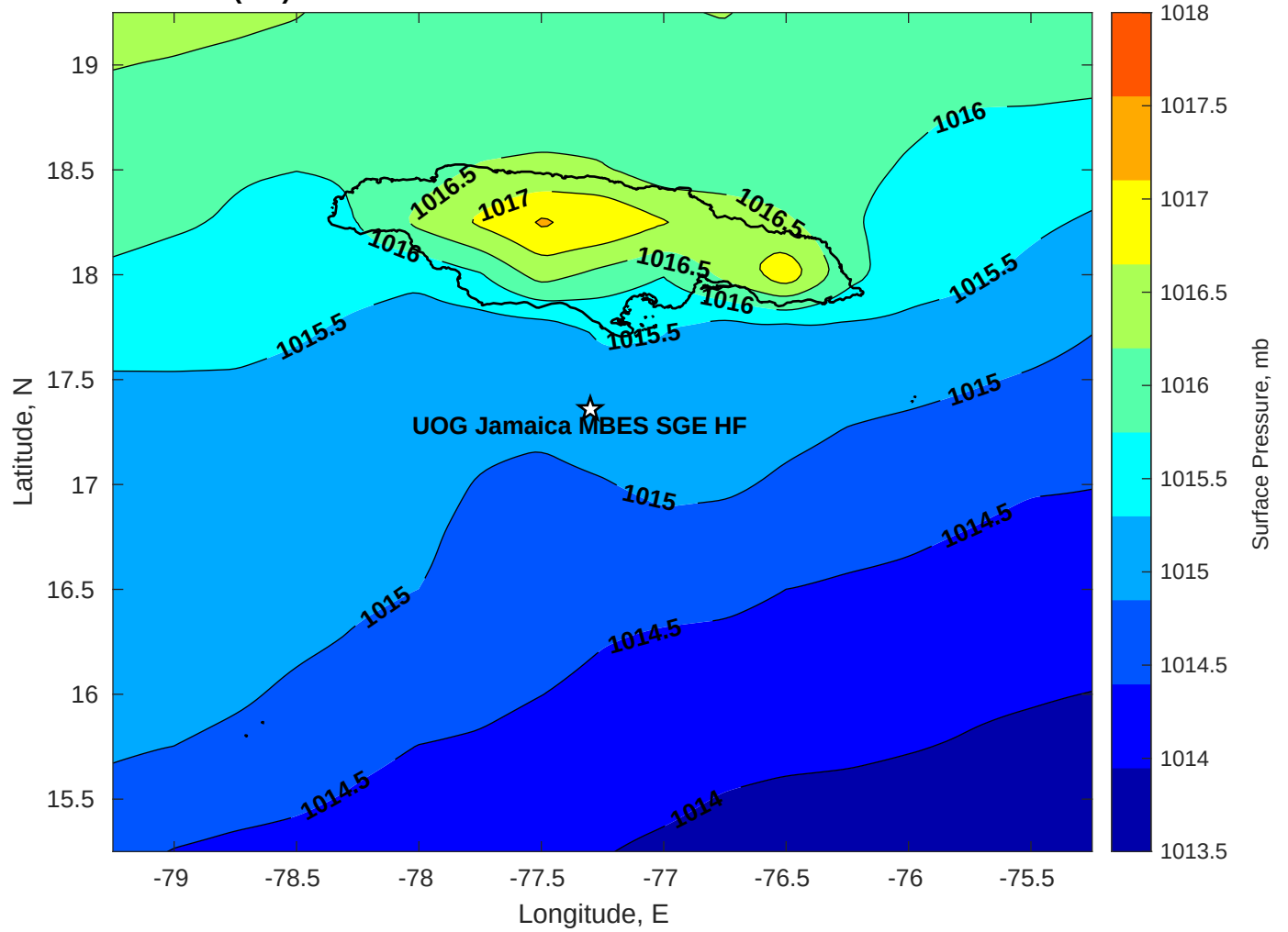
Surface Pressure (mb) for UOG Jamaica MBES SGE HF at 14-Feb-2026 06:00:00
