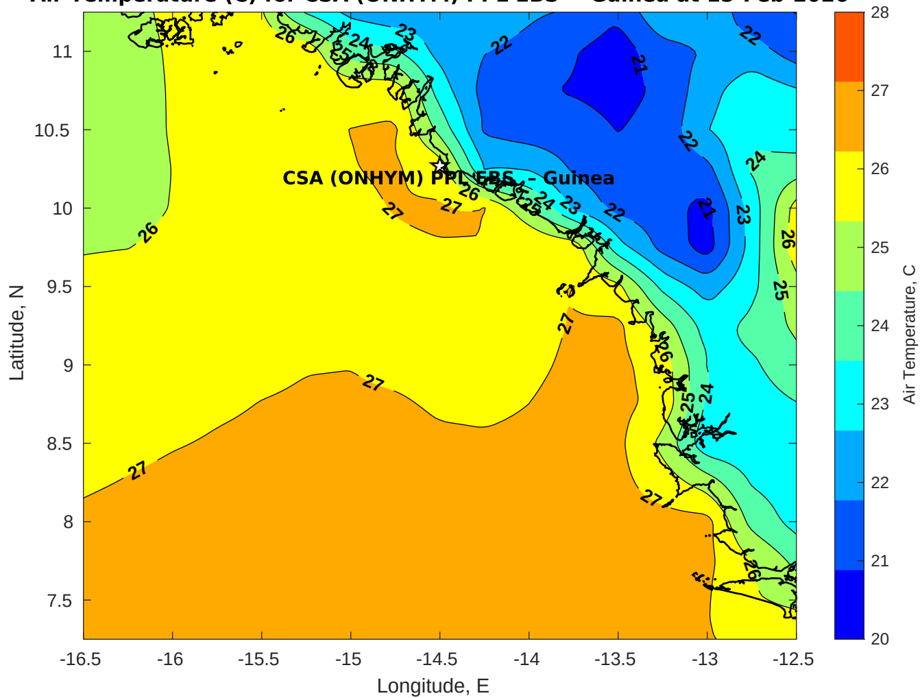
Air Temperature (C) for CSA (ONHYM) PPL EBS - Guinea at 15-Feb-2026
