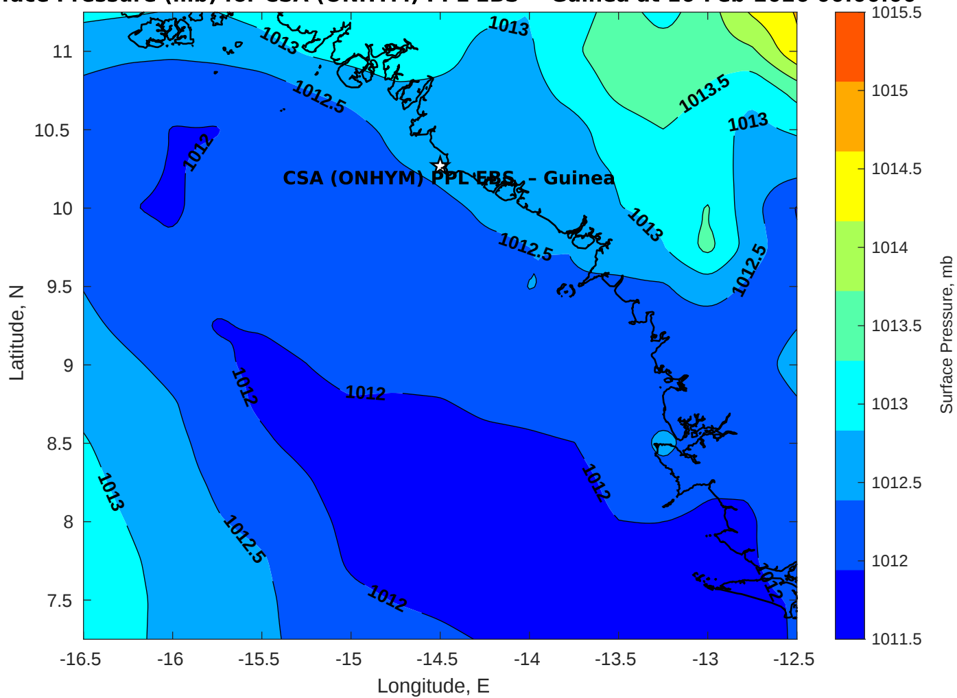
Surface Pressure (mb) for CSA (ONHYM) PPL EBS - Guinea at 16-Feb-2026 00:00:00
