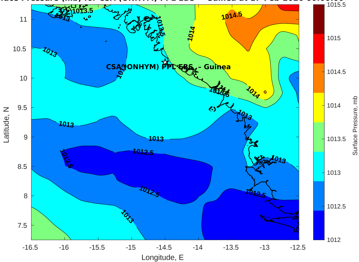
Surface Pressure (mb) for CSA (ONHYM) PPL EBS - Guinea at 17-Feb-2026 00:00:00
