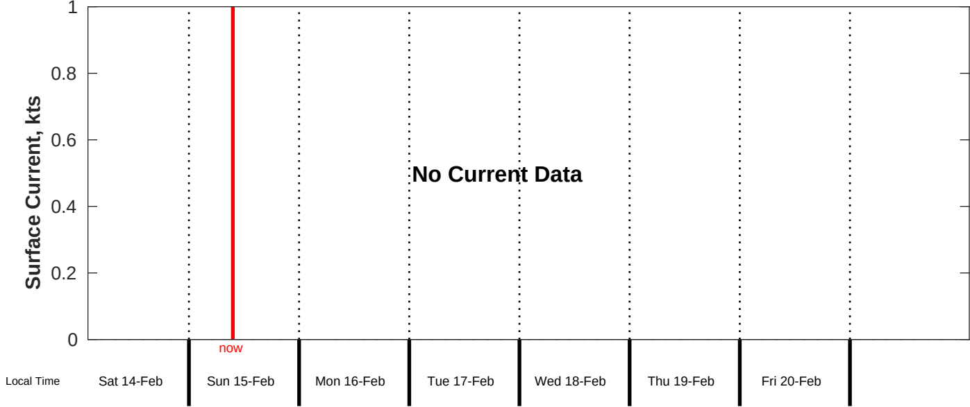
Surface Current Forecast for CSA (ONHYM) PPL EBS - Guinea from 14-Feb-2026 00:00:00 to 22-Feb-2026 00:00:00
