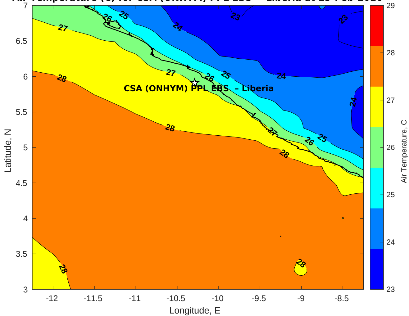
Air Temperature (C) for CSA (ONHYM) PPL EBS - Liberia at 15-Feb-2026
