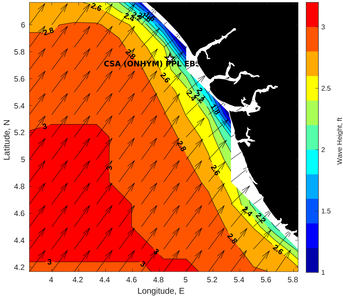
GFS Wave Height (ft) for CSA (ONHYM) PPL EBS - Nigeria at 15-Feb-2026 09:00:00
