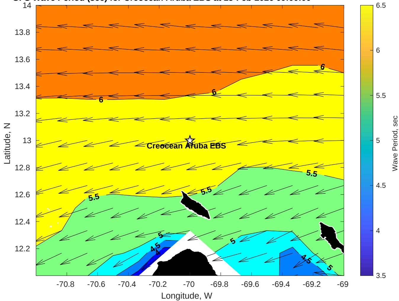
GFS Wave Period (sec) for Creoccean Aruba EBS at 15-Feb-2026 09:00:00
