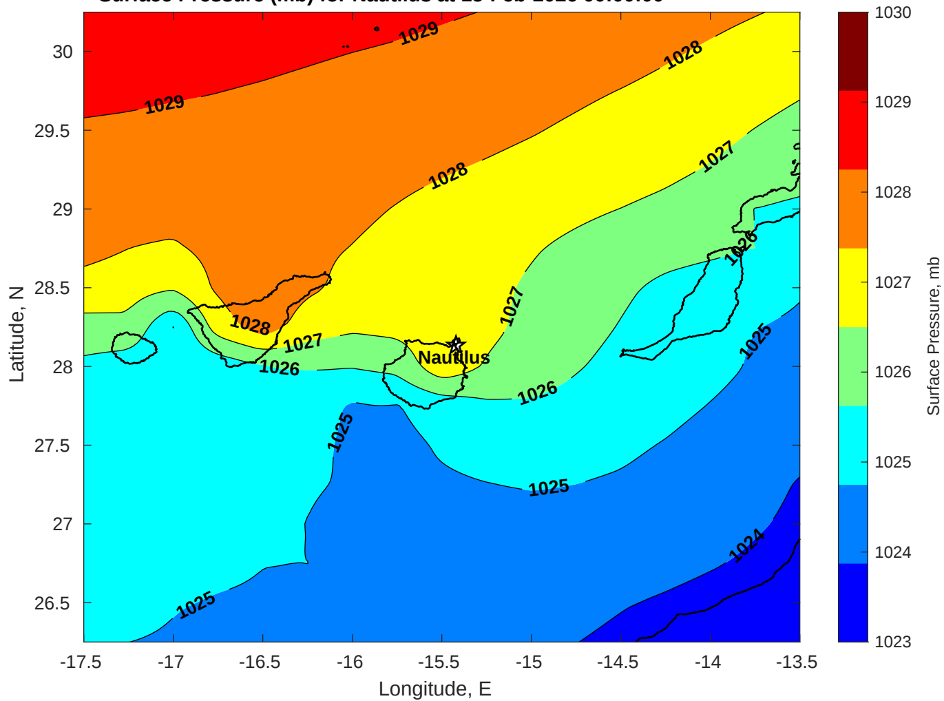
Surface Pressure (mb) for Nautilus at 15-Feb-2026 00:00:00
