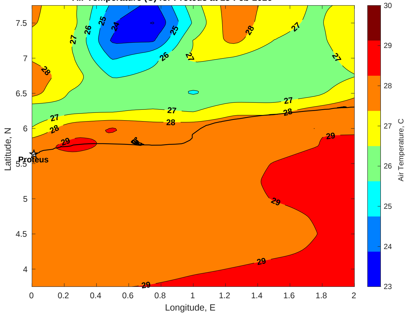
Air Temperature (C) for Proteus at 15-Feb-2026
