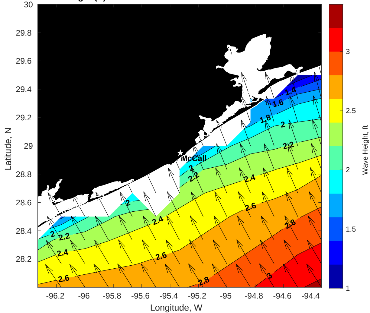
GFS Wave Height (ft) for Brooks McCall at 16-Feb-2026 09:00:00
