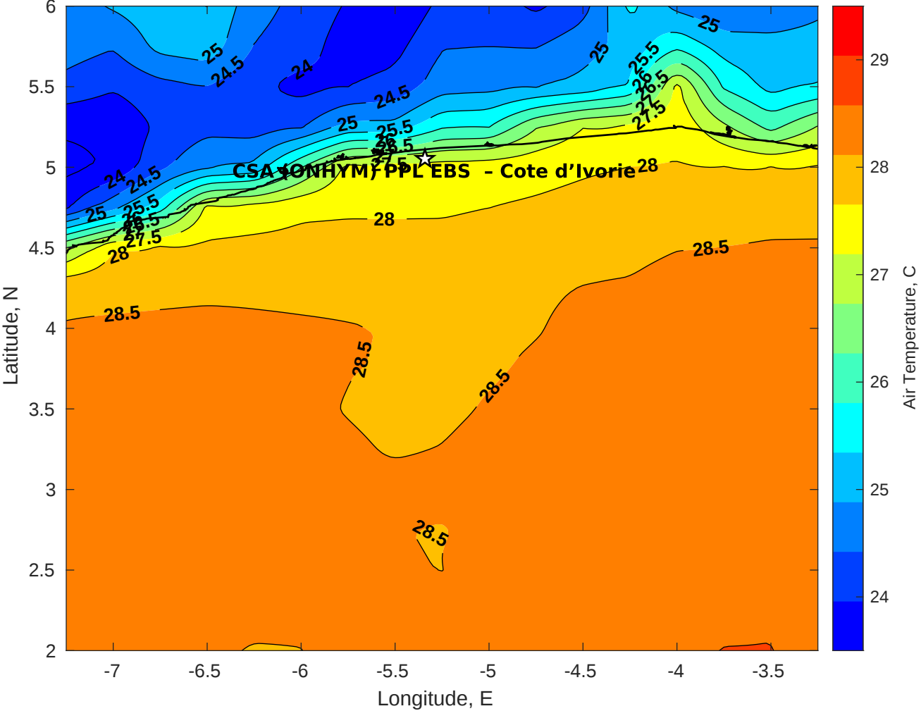
Air Temperature (C) for CSA (ONHYM) PPL EBS - Cote d'Ivoire at 16-Feb-2026
