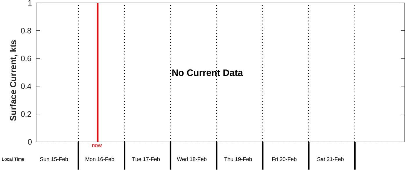
Surface Current Forecast for CSA (ONHYM) PPL EBS - Cote d'Ivoire from 15-Feb-2026 00:00:00 to 23-Feb-2026 00:00:00
