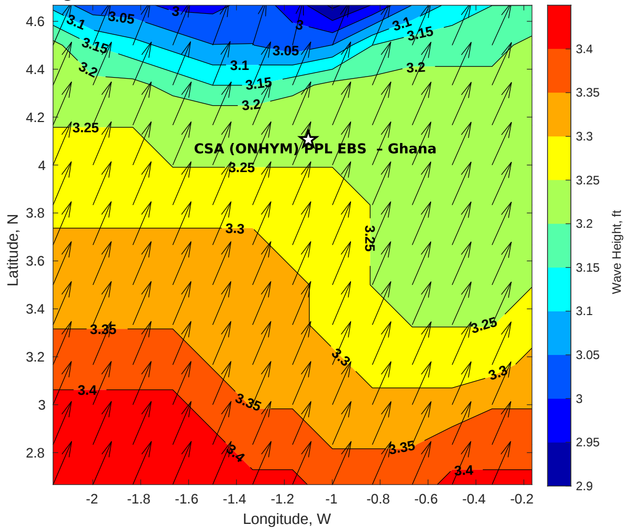
GFS Wave Height (ft) for CSA (ONHYM) PPL EBS - Ghana at 16-Feb-2026 09:00:00
