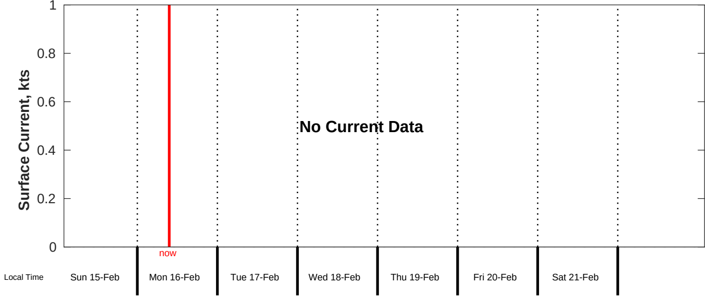
Surface Current Forecast for CSA (ONHYM) PPL EBS - Guinea from 15-Feb-2026 00:00:00 to 23-Feb-2026 00:00:00
