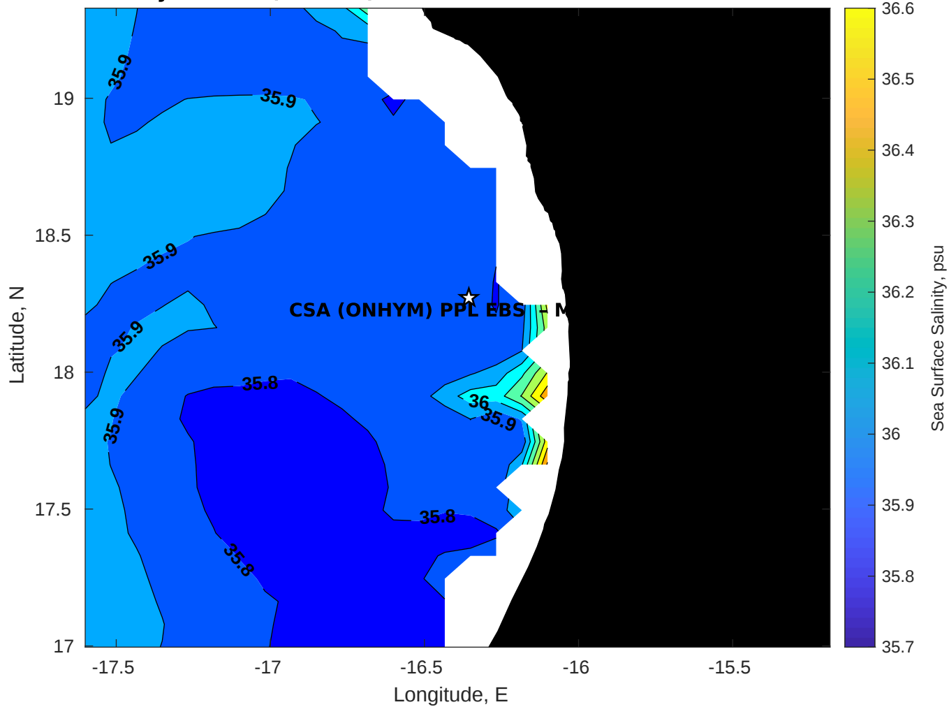
Surface Salinity for CSA (ONHYM) PPL EBS - Mauritania at 15-Feb-2026 00:00:00
