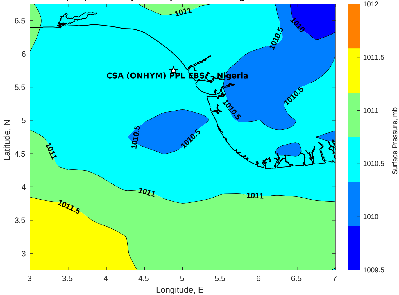
Surface Pressure (mb) for CSA (ONHYM) PPL EBS - Nigeria at 17-Feb-2026 00:00:00
