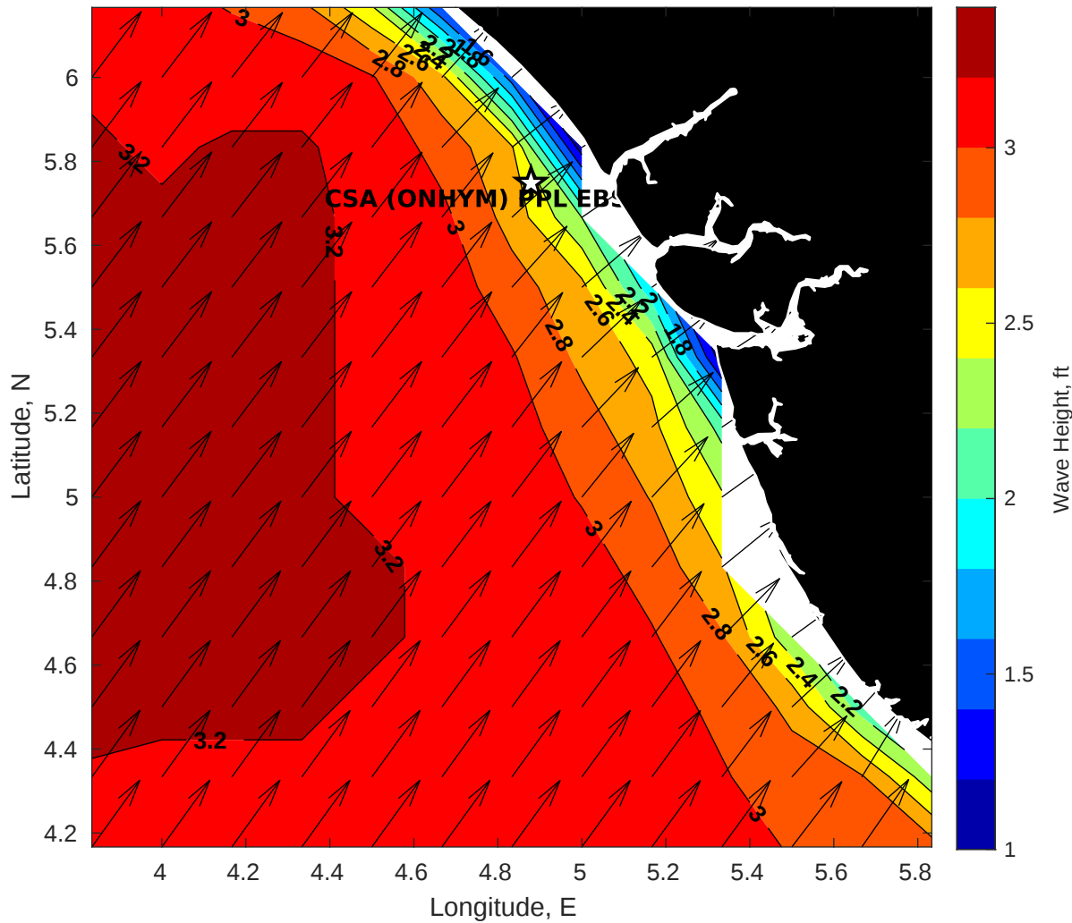
GFS Wave Height (ft) for CSA (ONHYM) PPL EBS - Nigeria at 16-Feb-2026 09:00:00
