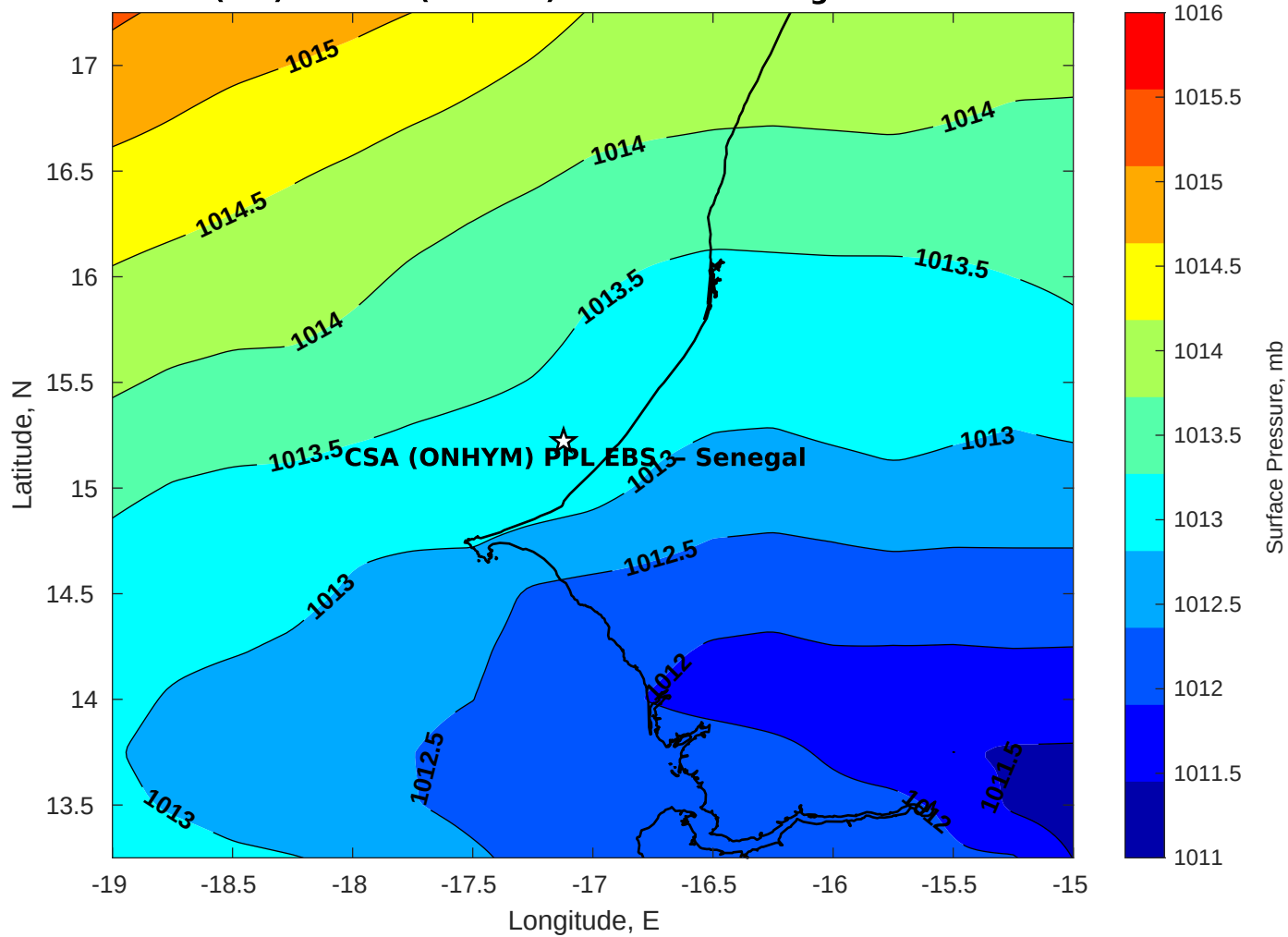
Surface Pressure (mb) for CSA (ONHYM) PPL EBS - Senegal at 18-Feb-2026 00:00:00
