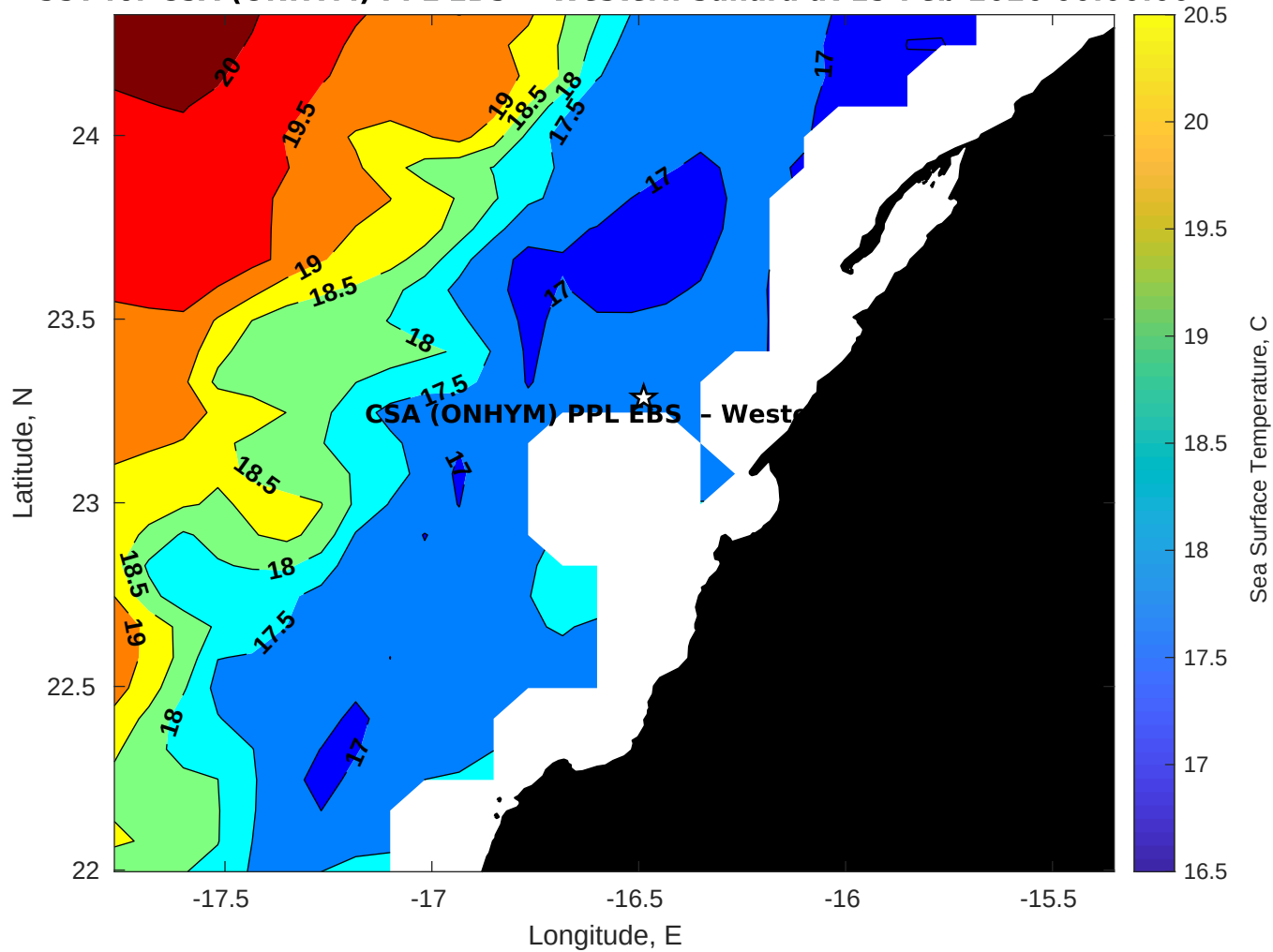
SST for CSA (ONHYM) PPL EBS - Western Sahara at 15-Feb-2026 00:00:00
