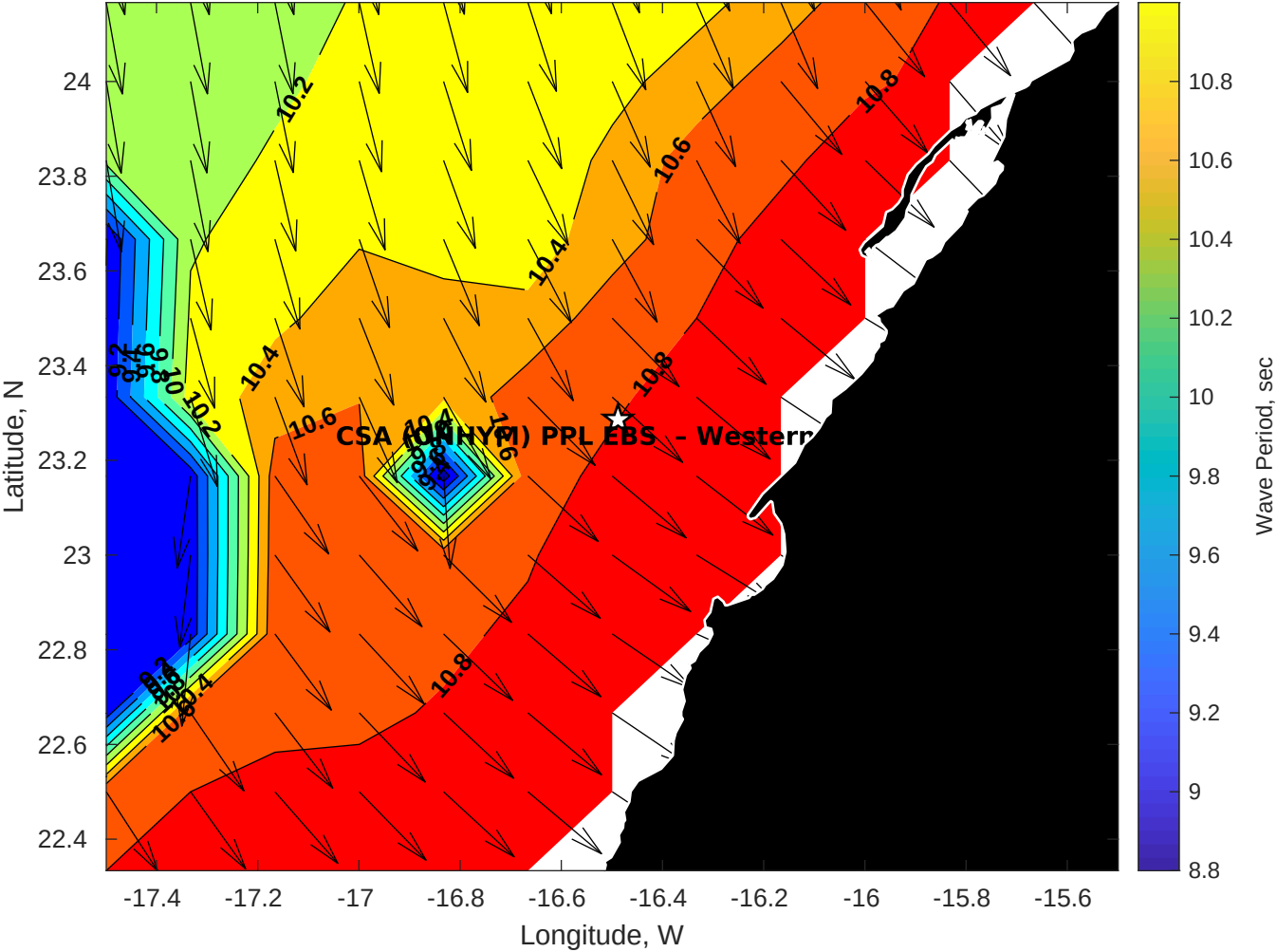
GFS Wave Period (sec) for CSA (ONHYM) PPL EBS - Western Sahara at 16-Feb-2026 09:00:00
