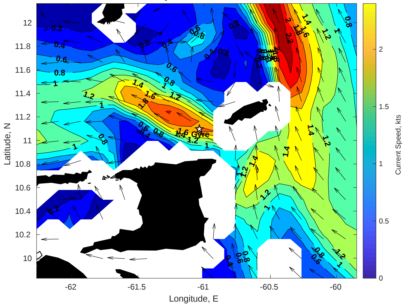
Surface Currents for Gyre at 15-Feb-2026 00:00:00
