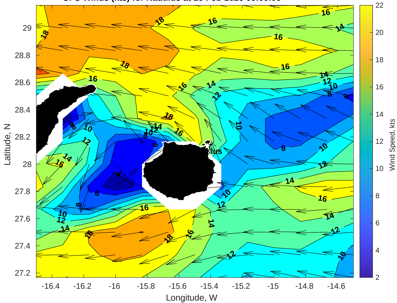
GFS Winds (kts) for Nautilus at 16-Feb-2026 09:00:00
