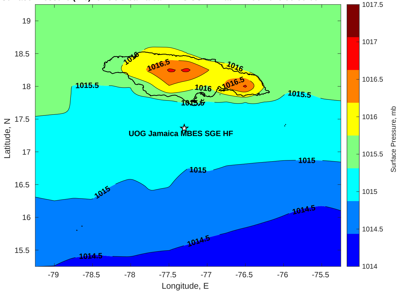
Surface Pressure (mb) for UOG Jamaica MBES SGE HF at 17-Feb-2026 06:00:00
