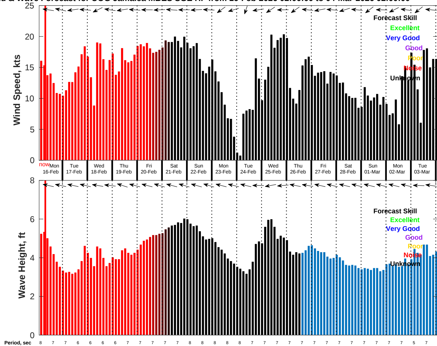
Wind & Wave Forecast for UOG Jamaica MBES SGE HF from 16-Feb-2026 02:00:00 to 04-Mar-2026 02:00:00
