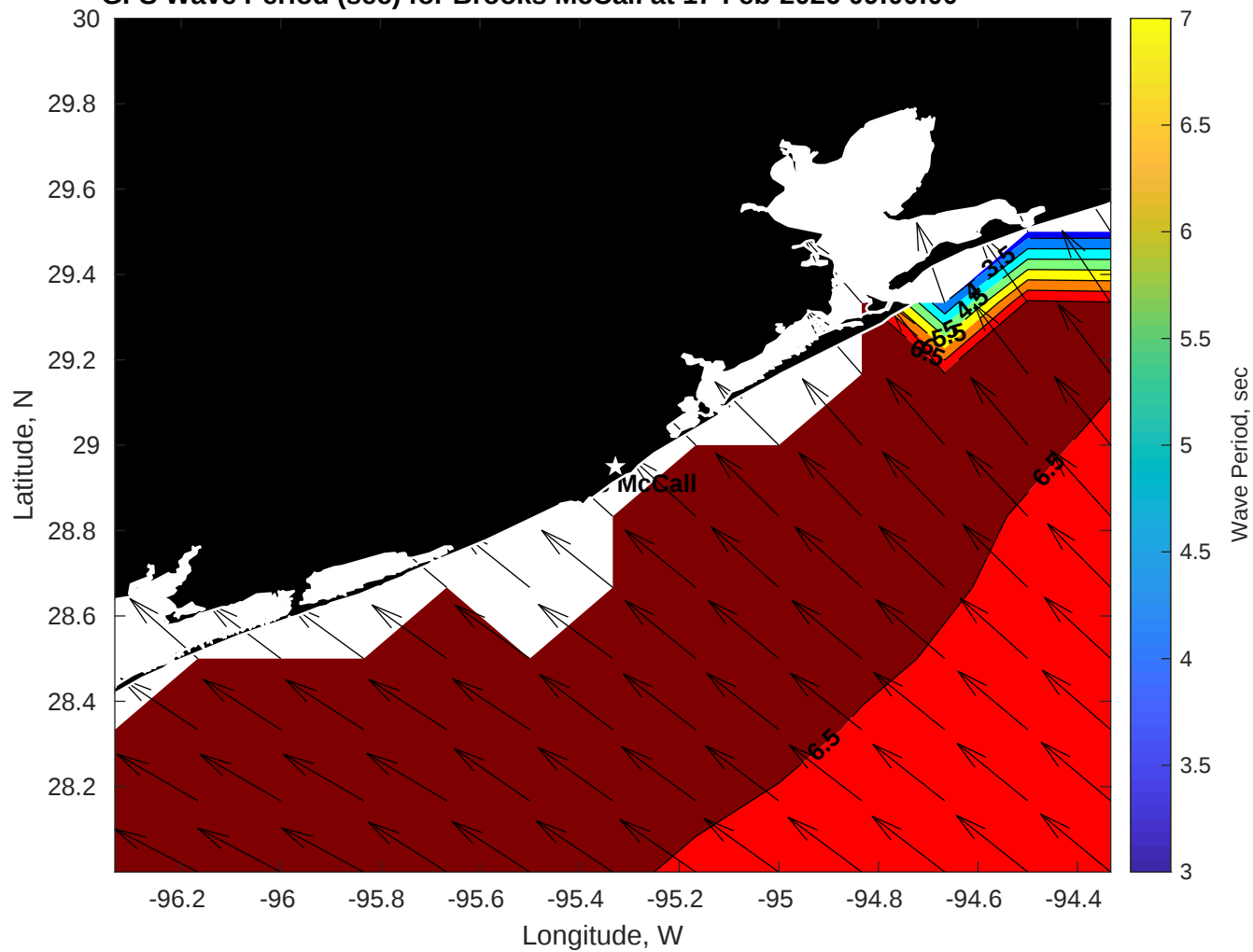
GFS Wave Period (sec) for Brooks McCall at 17-Feb-2026 09:00:00
