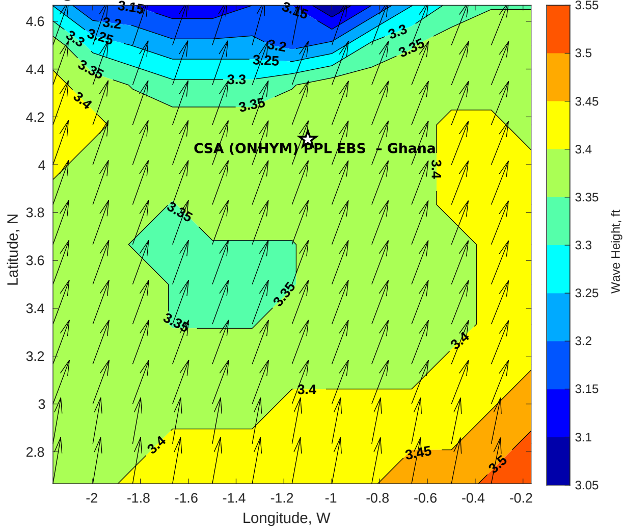
GFS Wave Height (ft) for CSA (ONHYM) PPL EBS - Ghana at 17-Feb-2026 09:00:00
