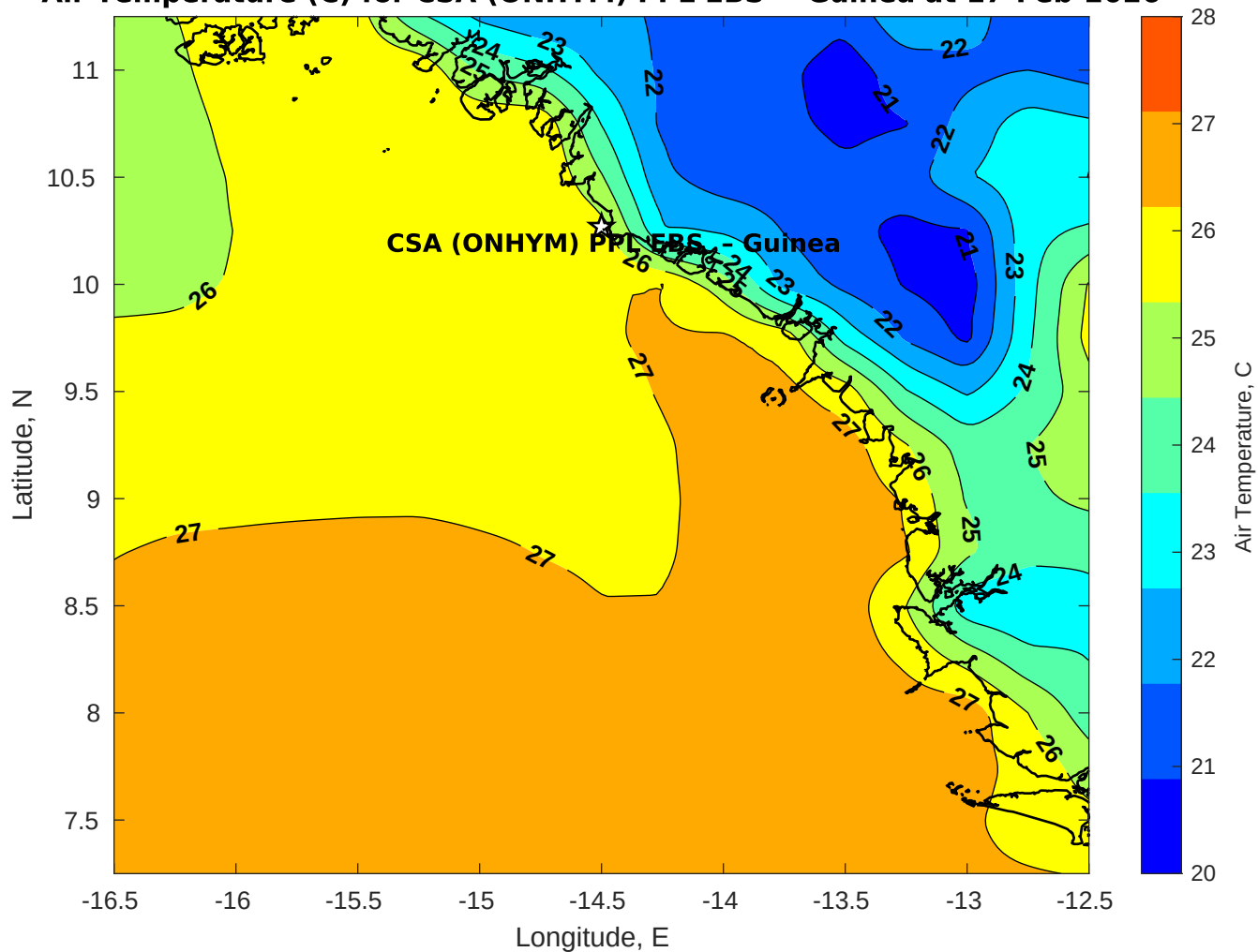
Air Temperature (C) for CSA (ONHYM) PPL EBS - Guinea at 17-Feb-2026
