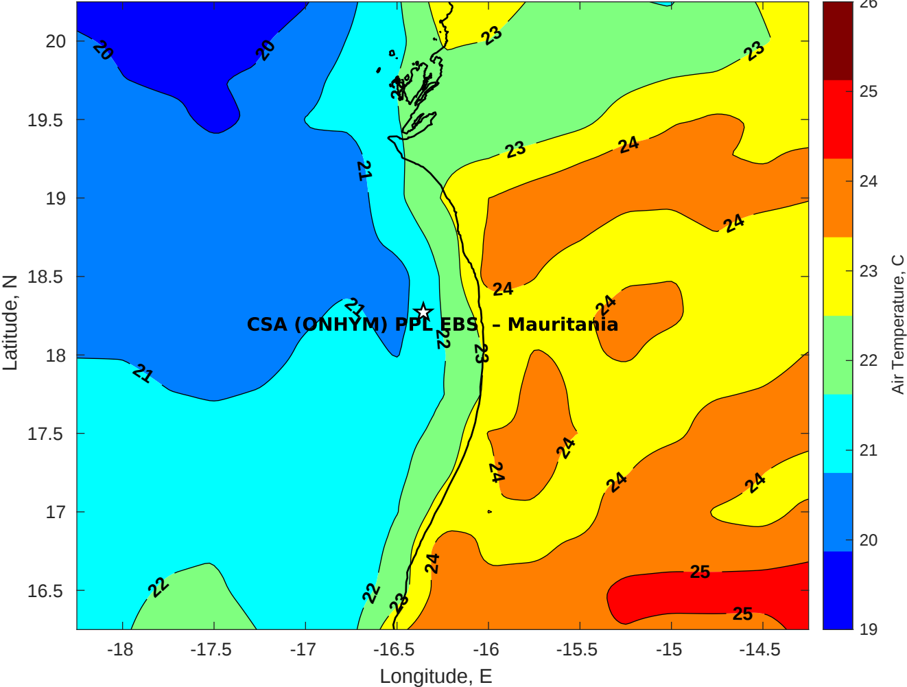
Air Temperature (C) for CSA (ONHYM) PPL EBS - Mauritania at 17-Feb-2026
