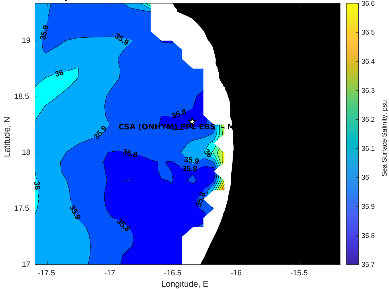
Surface Salinity for CSA (ONHYM) PPL EBS - Mauritania at 16-Feb-2026 00:00:00
